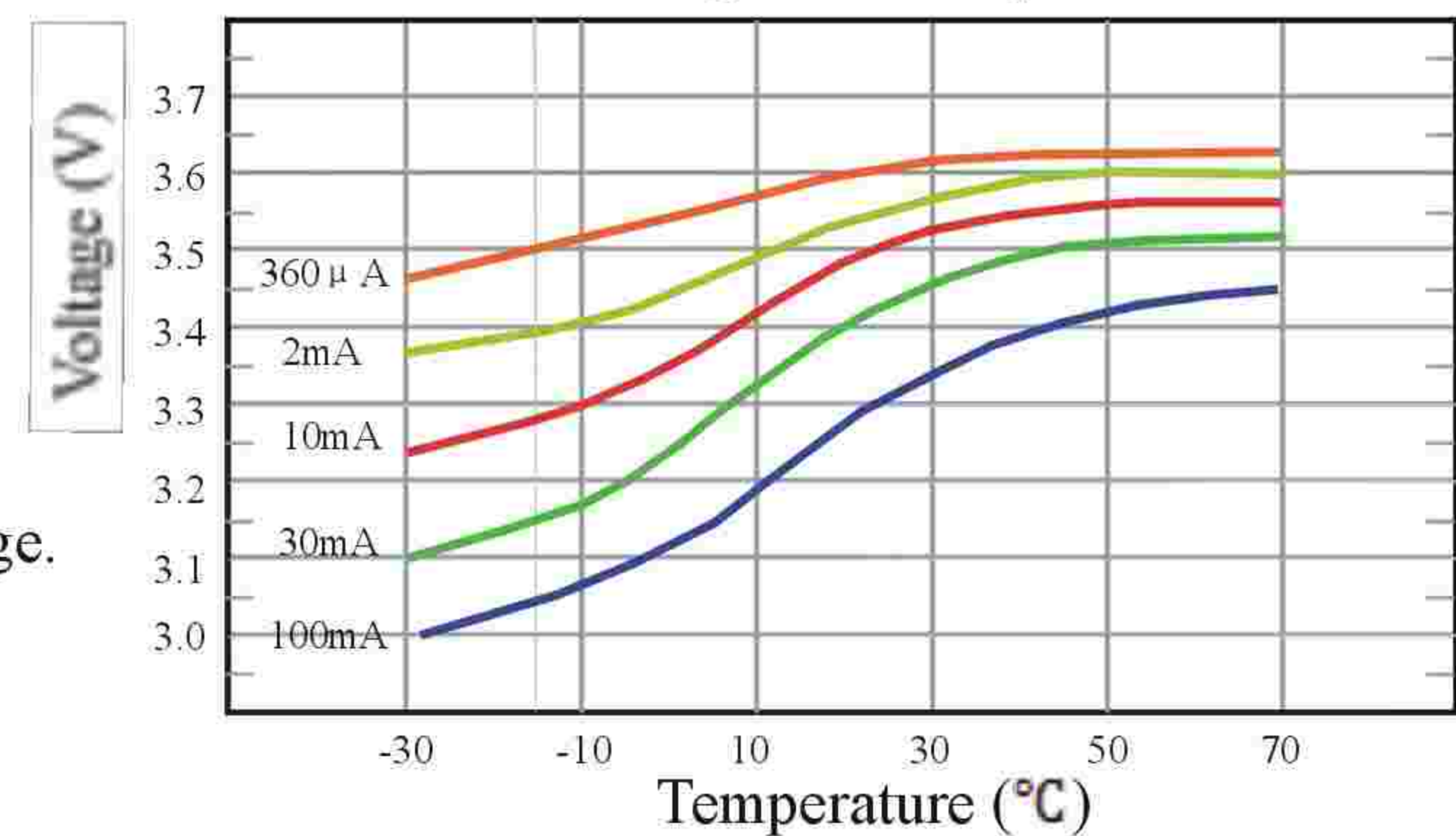
Voltage VS. Temperature
