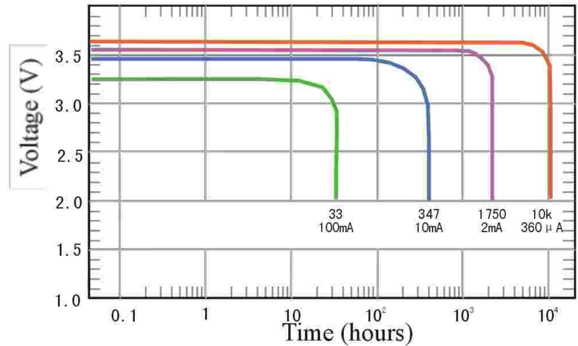
Capacity VS. Current
